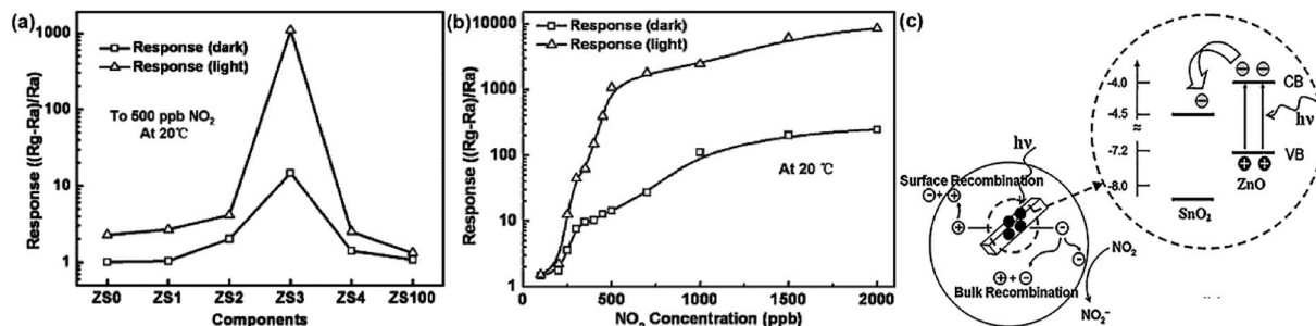
Fig. 12 (a) Responses of the sensor based on the composite materials with the various molar ratio of ZnO to \text{SnO}_2 to 500 ppb \text{NO}_2 at room temperature with and without UV light irradiation. (b) Response of the ZS3 sensor vs. \text{NO}_2 concentration at room temperature with and without UV light irradiation. (c) Schematic diagram: the carriers transport with UV light stimulated, energy band structure and electron–hole pair separation in the ZnO/ \text{SnO}_2 heterostructure in the area marked with a dashed circle. This figure has been reproduced with permission from ref. 131, Elsevier, Copyright 2012 (License Number: 4924100838478).
