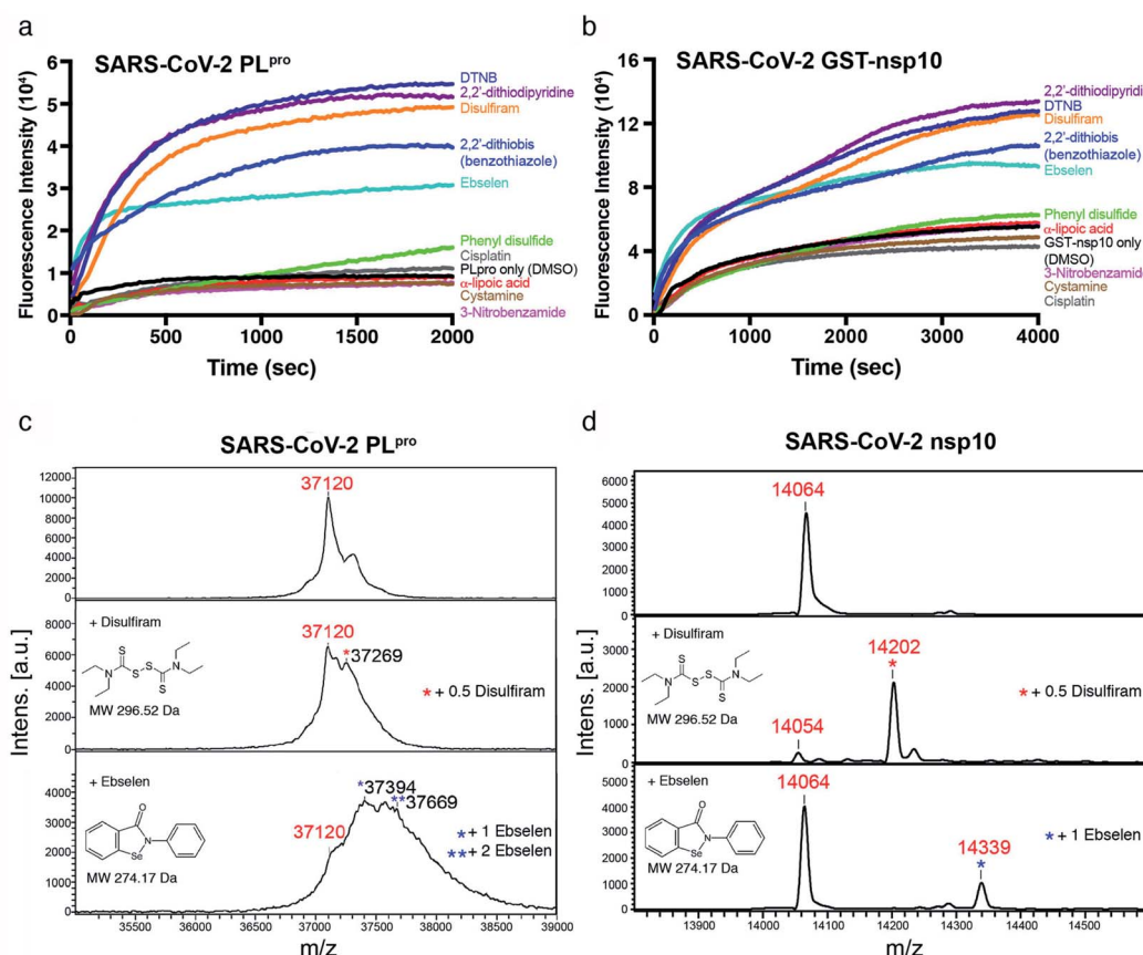
Fig. 2 \text{Zn}^{2+} release from SARS-CoV-2 PL pro and nsp10 by \text{Zn}^{2+} -ejecting compounds. Upon adding each \text{Zn}^{2+} -ejecting agent (5 \mu\text{M} ) to PL pro (5 \mu\text{M} ) (a), or GST-fused nsp10 (5 \mu\text{M} ) (b), \text{Zn}^{2+} release was detected by the increase of the fluorescence signal from FluoZin-3 (1 \mu\text{M} ) with emission and excitation wavelengths of 494 nm and 516 nm, respectively. The MWs of PL pro (c) and nsp10 (d) before (top) and after adding disulfiram (middle) or ebselen (bottom) were measured by MALDI-TOF mass spectrometry. Three independent experiments gave similar results hence only spectra from one of the experiments are shown.
