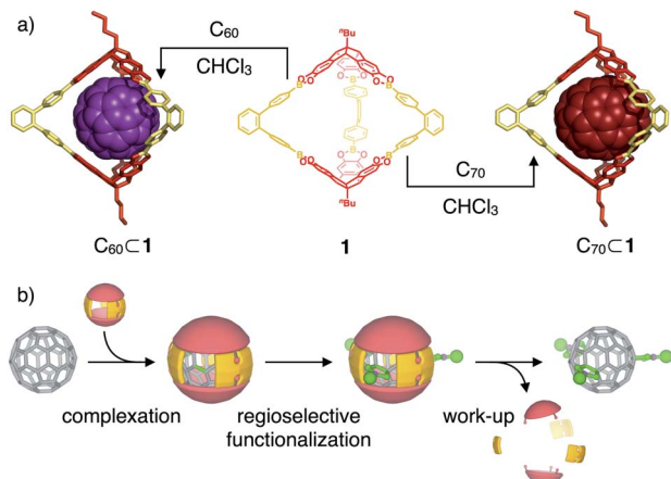
Fig. 1 (a) Supramolecular complexation of fullerenes C_{60} and C_{70} within the cavity of covalent organic boronate ester cage 1 (molecular structures of inclusion complexes are derived from semiempirical PM6 modeling); (b) schematic representation for the use of C_{60} -cage complexes as shadow masks for a regioselective exohedral C_{60} functionalization.
