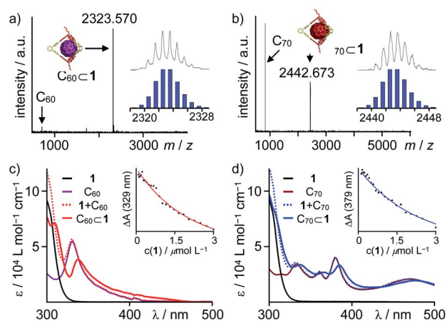
Fig. 2 MALDI-TOF MS (TCNQ, CHCl_3 ) for 1 : 1 mixtures of 1 and (a) C_{60} and (b) C_{70} (insets show comparison of measured and simulated isotope patterns); UV/Vis titration experiments for complex formation between 1 and (c) C_{60} (black 1 , purple C_{60} , dotted red 1 + C_{60} , red C_{60} @ 1 derived from global fit to 1 : 1 model, inset shows fit to 1 : 1 model at \lambda = 329 nm) and (d) C_{70} (black 1 , brown C_{70} , dotted blue 1 + C_{70} , blue C_{70} @ 1 derived from global fit to 1 : 1 model, inset shows fit to 1 : 1 model at \lambda = 379 nm).
