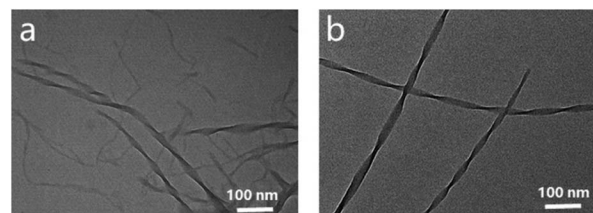
Fig. 4 TEM images of S -TPE-Ph-PEA assemblies from the DCM/HEX 1 : 9 system after self-assembly for 2 min (a) and 4 min (b), illustrating the formation and growth of helical fibers of S -TPE-Ph-PEA assemblies from solutions with a concentration of 1 \times 10^{-4} M.
