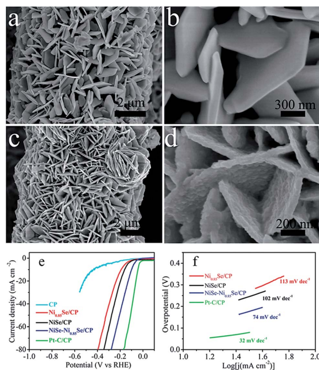
Fig. 8 (a and b) SEM image of NiO/CP. (c and d) SEM image of NiSe– \text{Ni}_{0.85}\text{Se}/\text{CP} . (e and f) HER LSVs and the Tafel slope of NiSe– \text{Ni}_{0.85}\text{Se}/\text{CP} in comparison with other studied catalysts in 1 M KOH. Reproduced with permission from ref. 74 (Copyright 2018 Wiley Publications).
