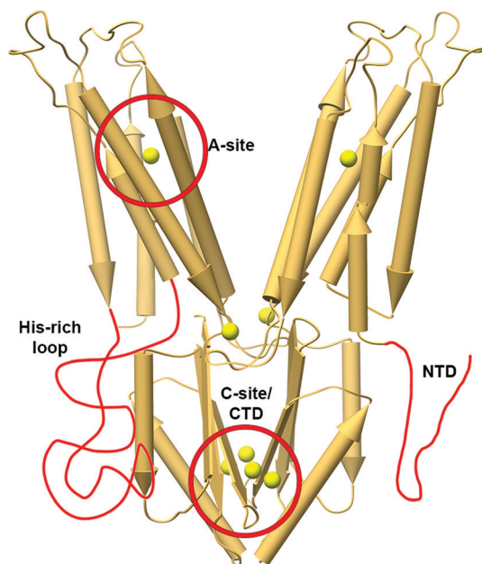
Fig. 5 The X-ray structure of YjiP (PDB code: 3H90 38 ) with features related to metal selectivity highlighted in red. The TM4-5 loop in YjiP is shorter than regular His-rich loops and it has a short NTD; hence, these features are drawn elongated for clarity. The locations of Zn 2+ ions in the structure are presented as enlarged yellow spheres.
