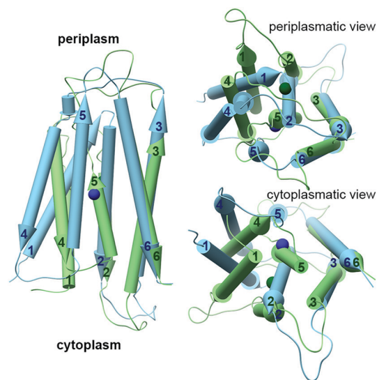
Fig. 3 The different conformations of monomeric TMDs of YjiPs. YjiP TMD monomers (EcYjiP, PDB code: 3H90, 38 in light green, and SoYjiP, PDB code: 5VRF, 36 in light blue) overlap onto each other, showing the movement of TMH1,2,4,5 with respect to TMH3,6 in the transition between the inward facing (SoYjiP) and outward facing (EcYjiP) conformations. The \text{Zn}^{2+} ions are presented in the protein's darker colors.
