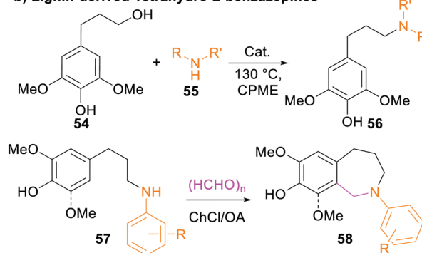
Scheme 5 (a) Cleavage pathways of lignin through acidolysis followed by in situ conversion into stable products. (b) Construction of lignin-derived tetrahydro-2-benzazepines 58 . 60,269
