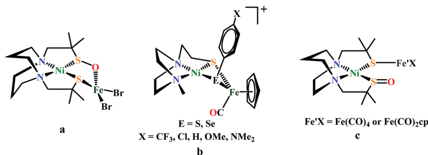
Fig. 34 Only known \text{NiFe} -complexes studied as a \text{O}_2 -tolerant [\text{NiFe}] -hydrogenase mimics.
