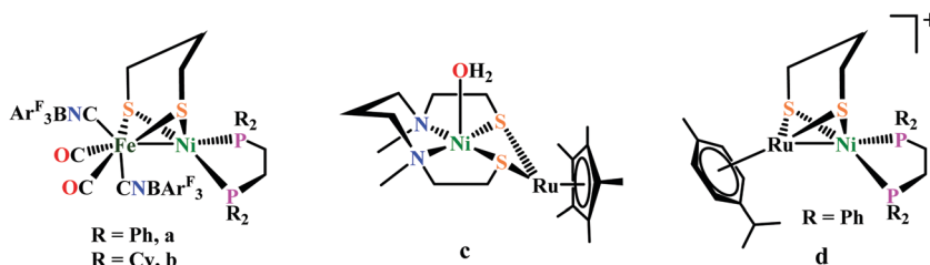
Fig. 33 Selected examples of [\text{NiFe}] -hydrogenase mimics active for \text{H}_2 activation.
