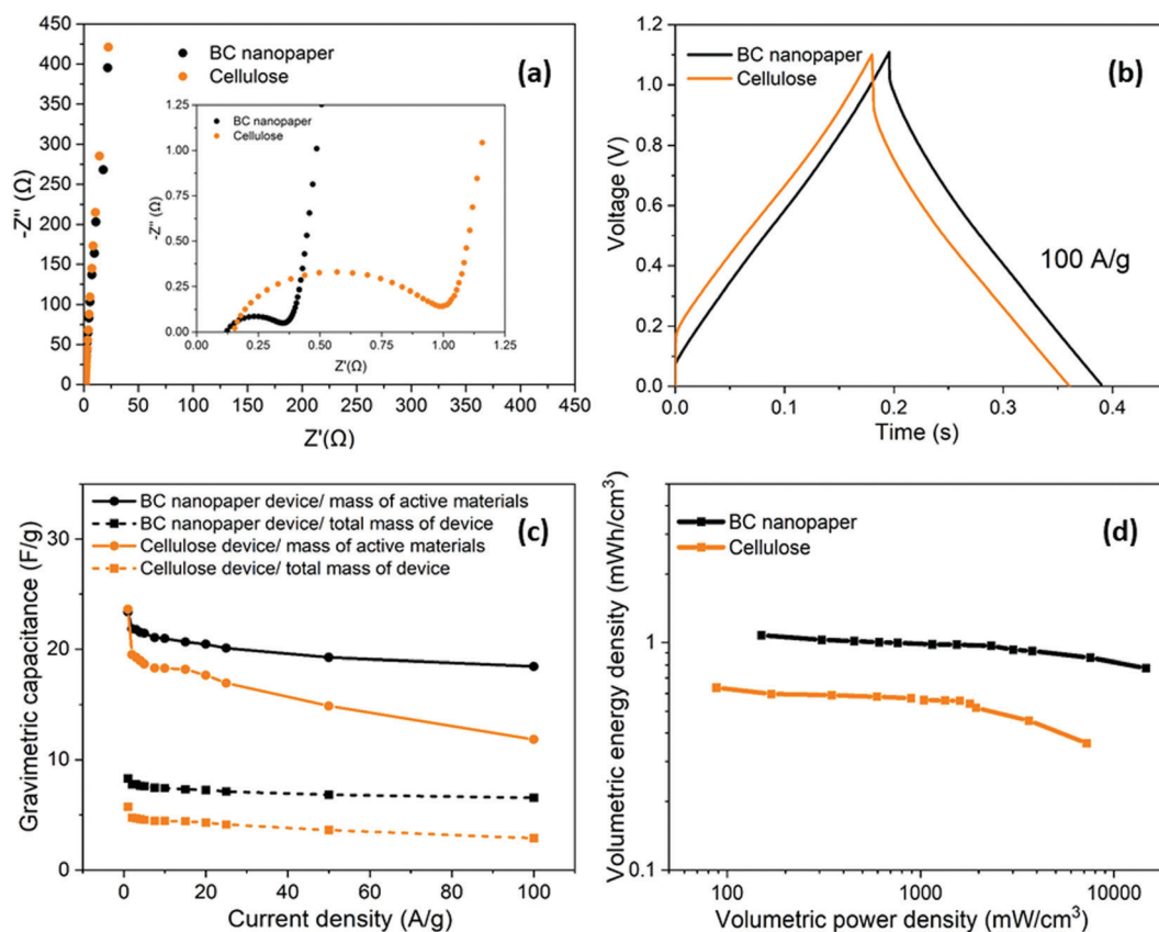
Fig. 4 Full-cell electrochemical performance of aqueous symmetric supercapacitors using nanotubule buckypaper electrodes sandwiched with BC nanopaper (black) and cellulose (orange) as separators: (a) Nyquist plots and (b) GCD curves at 100 A \text{g}^{-1} , (c) the calculated gravimetric capacitance normalised by both active material (straight line) and total mass of device (dash line) and (d) volumetric Ragone plots normalised by total mass of device.
