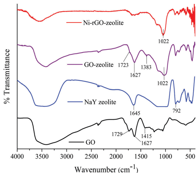
Fig. 1 FT-IR spectra of GO, NaY zeolite, GO-zeolite and Ni-rGO-zeolite.
