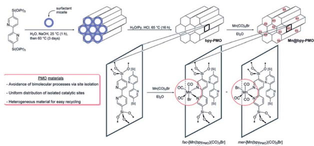
Fig. 16 Synthesis pathway to [Mn(bpy PMO )(CO) 3 Br]. 116 Reproduced from ref. 116 with permission from the Royal Society of Chemistry.
