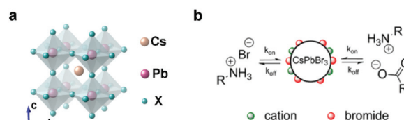
Fig. 1 (a) Schematic of the cubic perovskite lattice. (b) Schematic representation of the dynamic surface stabilization by oleylamine bromide, oleylamine oleate and OLA. Reproduced with permission from ref. 39. Copyright 2016 American Chemistry Society.
