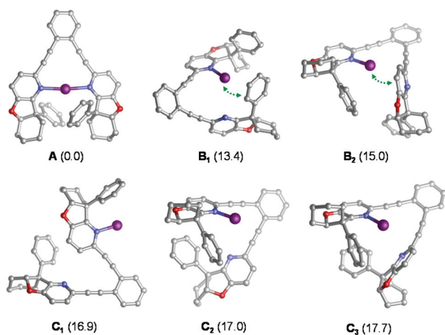
Fig. 3 Various forms of complex [2-1] + as obtained from DFT calculations. Relative stabilities are given in kcal mol -1 with respect to the symmetric chelating form. Hydrogen atoms are omitted for clarity. Close I + – \pi contacts in B 1 and B 2 are highlighted with green dotted arrows.
