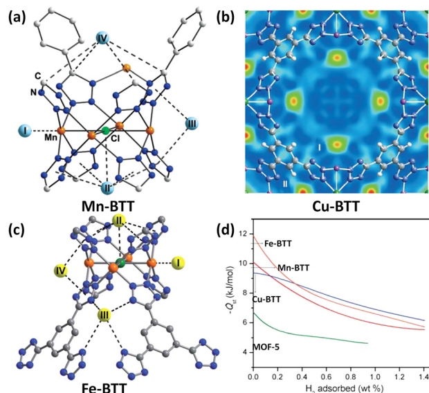
Fig. 4 \text{D}_2 binding sites in (a) Mn-BTT, (b) Cu-BTT and (c) Fe-BTT compounds as determined by the NPD experiment with the \text{D}_2 loadings of 12, 30 and 20 per formula unit, respectively, and (d) comparison of their \text{H}_2 adsorption heats. Reprinted with permission from ref. 36, 38 and 39. Copyright 2006, American Chemical Society; Copyright 2007, Wiley; Copyright 2010, Royal Society of Chemistry.
