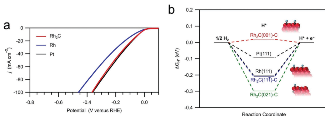
Fig. 65 (a) The HER polarisation curves of 20 wt% \text{Rh}_2\text{C}/\text{C} (red), Pt/C (black), and Rh/C (blue). The data were recorded in a 1.0 M KOH electrolyte with a scan rate of 50 \text{ mV s}^{-1} . (b) The 3-state free energy diagram for HER. The structural models show the \text{OH}^* pre-covered surfaces used for calculations. The blue spheres are hydrogen atoms, and the gray spheres are oxygen atoms. Reproduced with permission from ref. 1003. Copyright American Chemical Society 2020.
