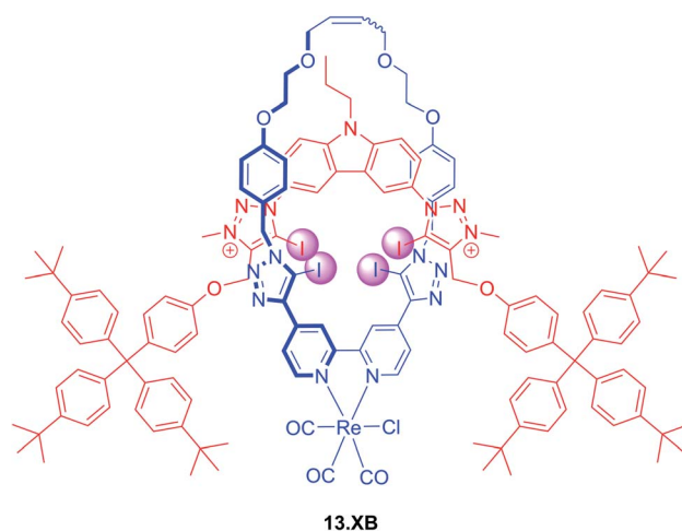
Fig. 16 All XB \text{Re}(\text{I})(\text{CO})_2\text{Cl} -containing [2]rotaxane 13.XB for selective fluorescent halide sensing in ACN/ \text{H}_2\text{O} mixtures.
