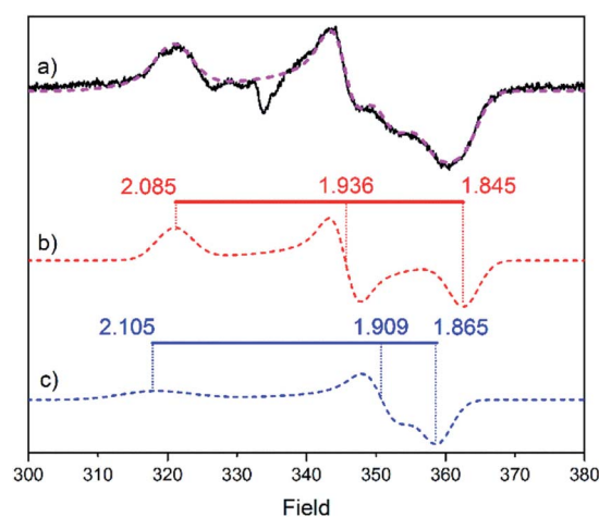
Fig. 3 EPR spectrum recorded on a 2-HydA1 (150 \mu\text{M} ) in 100 mM Tris buffer pH 8 + 200 mM KCl. (a) Experimental data (black) is overlaid with the simulated spectrum (pink dashed line) obtained fitting two rhombic signals. (b) Simulated spectrum of the first rhombic signal ( g_{\text{zyx}} = 2.085\ 1.936\ 1.845 ). (c) Simulated spectrum of the second rhombic signal ( g_{\text{zyx}} = 2.105\ 1.909\ 1.865 ). Experimental parameters: frequency: 9.365\text{ GHz} , temperature = 10\text{ K} ; microwave power = 64\ \mu\text{W} .
