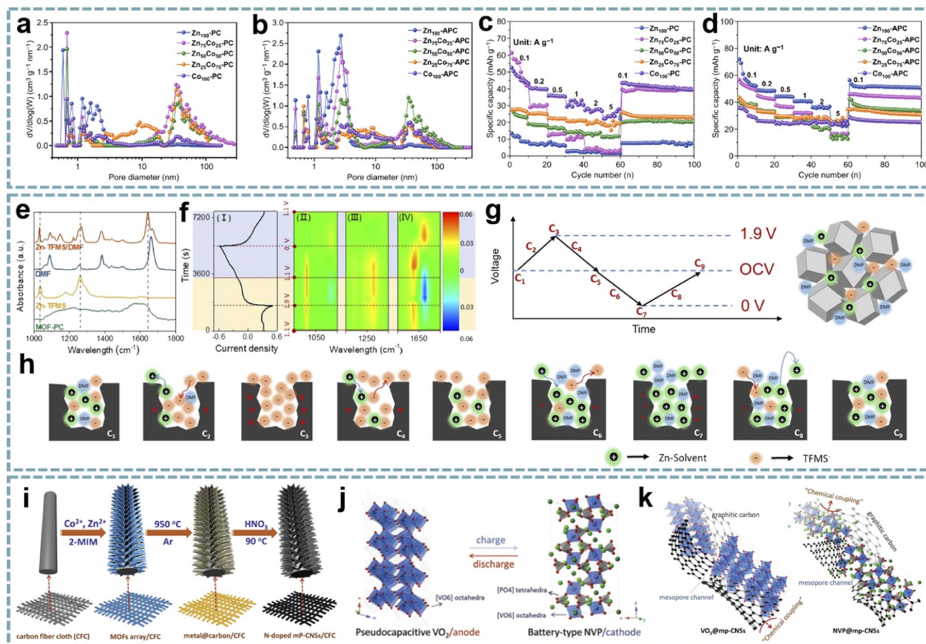
Fig. 7 MOF-derived porous carbons for MIHCs. Pore size distribution curves of (a) \text{Zn}_x\text{Co}_{100-x}\text{-PCs} and (b) \text{Zn}_x\text{Co}_{100-x}\text{-APCs} . Rate capabilities at different current densities of (c) \text{Zn}_x\text{Co}_{100-x}\text{-PCs} and (d) \text{Zn}_x\text{Co}_{100-x}\text{-APCs} . Reproduced with permission from ref. 160. Copyright 2020, Springer. (e) FT-IR spectra of neat DMF, Zn-TFMS, MOF-PC, and Zn-TFMS/DMF electrolytes. (f) CV curve (I) at 0.5 \text{ mV s}^{-1} ; 2D color-filled contour plots (II, III, and IV) from the in situ ATR-FTIR test of the ZIHC. (g, h) The reaction process schematic diagram of the adsorption/desorption of ions in the MOF-PC electrode in a Zn-TFMS/DMF electrolyte. Reproduced with permission from ref. 161. Copyright 2021, Wiley-VCH. (i) Schematic diagram of the fabrication of N-doped mesoporous graphitic carbon nanosheet arrays. (j) Schematic illustration of the NIC device using flexible \text{VO}_2\text{@mp-CNSs/CFC} and \text{NVP@mp-CNSs/CFC} electrodes as the anode and cathode. (k) Schematic illustration of \text{Na}^+ storage of \text{VO}_2\text{@mp-CNSs/CFC} and \text{NVP@mp-CNSs/CFC} . Reproduced with permission from ref. 70. Copyright 2018, Wiley-VCH.
