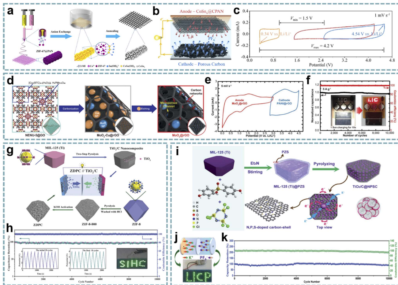
Fig. 10 MOF-derived metal/carbons for MIHCs. (a) Schematic diagram of the fabrication process of CoSn 4 @CPAN nanofibers. (b) Schematic of the configuration of a full-cell LIHC. (c) CV profiles from a three-electrode device. Reproduced with permission from ref. 189. Copyright 2020, Elsevier. (d) Schematic diagram of the fabrication process of the MoO 2 @rGO anode. (e) CV curves of the MoO 2 @rGO anode and PANI@rGO cathode at a scan rate of 5 mV s -1 . (f) Charge–discharge cycling stability at 5 A g -1 with a wireless charging kit charged by a solar cell. Reproduced with permission from ref. 78. Copyright 2020, Wiley-VCH. (g) Construction process of the TiO 2 /C anode and ZDPC cathode. (h) Cycling performance and coulombic efficiency of the TiO 2 /C//ZDPC SIHC under 1 A g -1 . Reproduced with permission from ref. 193. Copyright 2018, Wiley-VCH. (i) Schematic diagram of the preparation process of TiO 2 /C@NPSC. (j) LED arrays powered by the PIHC device. (k) Cycling performance and coulombic efficiency. Reproduced with permission from ref. 80. Copyright 2020, Royal Society of Chemistry.
