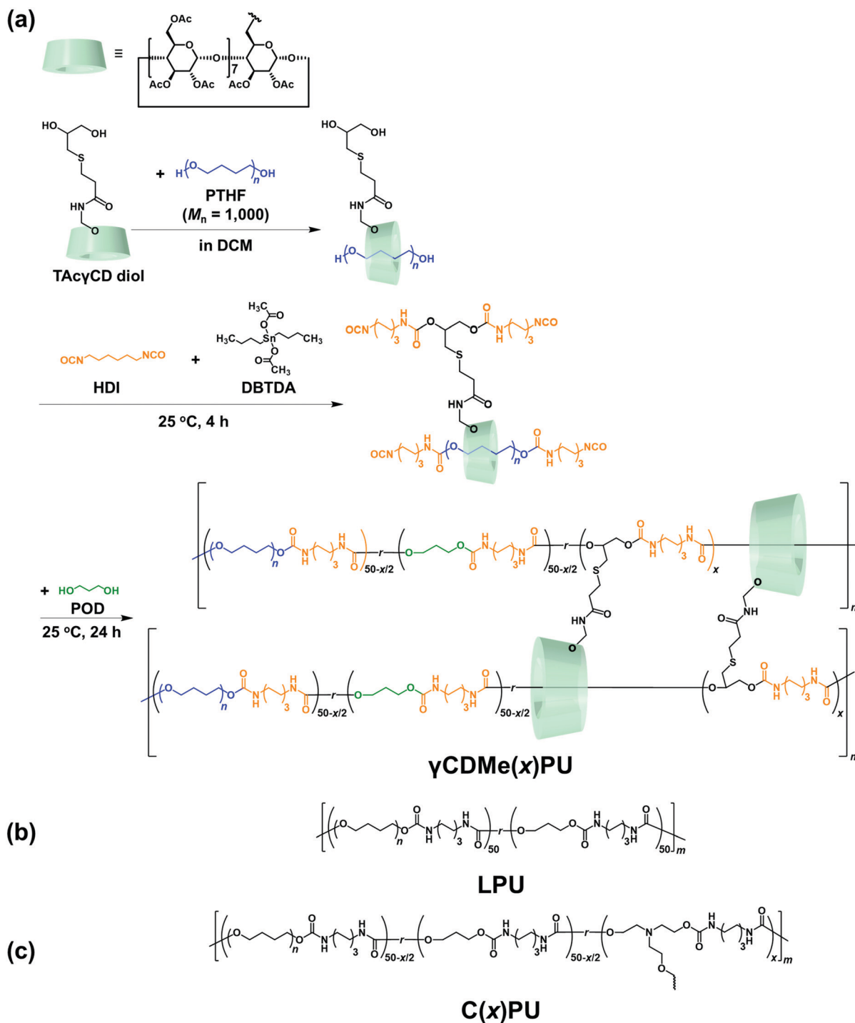
Fig. 1 (a) Synthesis of \gamma\text{CDMe}(x)\text{PU} and chemical structures of (b) LPU and (c) \text{C}(x)\text{PU} , where x refers to the molar ratio of TAc \gamma\text{CD} diol monomer or TEA monomer.
