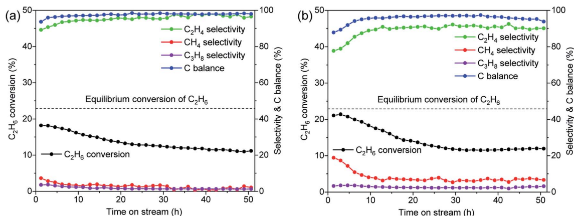
Fig. 8 Catalytic performances of (a) 0.5Co@MFI and (b) 1.3Co@MFI catalysts at 7.5 bar pressure. Reaction conditions: 50 mg catalyst, pretreatment by 10% H 2 /N 2 for 30 min, 20% C 2 H 6 /N 2 , 5 mL min -1 , 650 °C.
