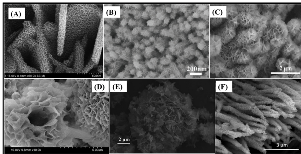
Fig. 6 SEM images of (A) porous \text{ZnCo}_2\text{O}_4/\text{MnO}_2 heterostructures/NF, 108 (B) \text{ZnCo}_2\text{O}_4@/\text{MnO}_2 nanowires/NF, 115 (C) mesoporous \text{ZnCo}_2\text{O}_4/\text{NiO} flower-like clusters/NF, 111 (D) \text{ZnCo}_2\text{O}_4@/\text{CdS} nanoflowers/NF, 116 (E) hydrangea-like \text{ZnCo}_2\text{O}_4/\text{Ni}_3\text{V}_2\text{O}_8 nanostructures/NF 107 and (F) \text{ZnCo}_2\text{O}_4@/\text{Ni}_3\text{S}_2 heterostructured nanowires/NF. 117 Panel A: Reproduced with permission. 108 Copyright © 2018 Elsevier Ltd. All rights reserved. Panel B: Reproduced with permission. 115 Copyright Marketplace™, Royal Society of Chemistry. Panel C: Reproduced with permission. 111 Copyright © 2018 Elsevier Ltd. All rights reserved. Panel D: Reproduced with permission. 116 Copyright © 2020 Korean Physical Society. Published by Elsevier B.V. All rights reserved. Panel E: Reproduced with permission. 107 Copyright © 2019 Elsevier Ltd and Techna Group S.r.l. All rights reserved. Panel F: Reproduced with permission. 117 Copyright © 2017 Elsevier B.V. All rights reserved.
