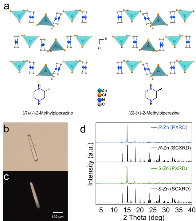
Fig. 1 (a) Crystal structures of R - and S -Zn. (b) Optical microscope image and (c) the corresponding crossing polarized microscope image of an R -Zn crystal. (d) Powder XRD patterns of R - and S -Zn.
