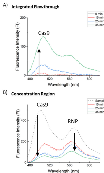
Fig. 5 Fluorescence emission spectra for integrated flowthrough fraction and concentration region fraction with excitation at 440 nm and Cy2-Cas9 emission maximum at 510 nm. Samples were collected for concentration trials of 15, 25 and 35 minutes, as well as a 0.1× PBS sample (‘0 minute’ sample for integrated flowthrough) and a RNP sample (0 minute ‘sample’ for concentration region). A) In the flowthrough we see a 25× increase in the Cas9 intensity from 15 to 25 minutes, and 25% of the initial sample (0 min sample) recovered in the flowthrough. B) In the concentrated region we see a 63% decrease in Cas9 intensity from 15 minutes to 35 minutes, with an 88% decrease in fluorescence intensity from the initial sample.
