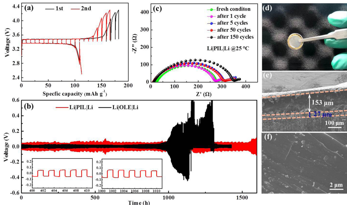
Fig. 4 (a) GITT curves of Li|LFP batteries with PIL membrane; (b) galvanostatic cycling performance of Li symmetrical battery, insets: partially enlarged images at a different time; (c) Nyquist plots of the symmetric Li battery with PIL membrane at various cycles; (d) digital photo of systematic battery after cycling; (e) cross-sectional SEM image of the Li|PIL|LFP battery after cycling; (f) top-view SEM image of the Li anode with PIL electrolyte after cycling.
