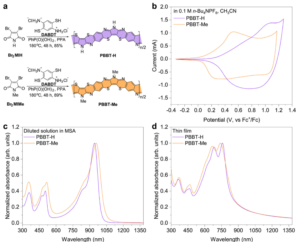
Fig. 1 Synthesis and physicochemical properties of PBBT-H and PBBT-Me. (a) Synthetic route of PBBT-H and PBBT-Me. (b) CV of PBBT-H and PBBT-Me in 0.1\text{ M } n\text{-Bu}_4\text{NPF}_6 acetonitrile solution. (c) and (d) UV-vis-NIR absorption spectra of PBBT-H and PBBT-Me in diluted MSA solutions (c) and thin films (d).
