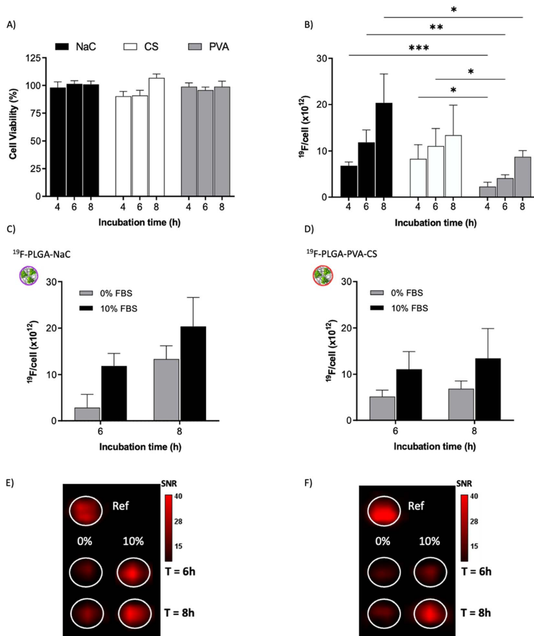
Fig. 3 Labelling efficiency. (A) Cell viability of labeled BV2 cells (normalized to the cell survival of unlabeled cells, ctrl) evaluated by standard trypan blue staining after 4, 6 and 8 h of incubation with the different ^{19}\text{F} -PLGA-NPs. (B) ^{19}\text{F} cellular uptake as a function of incubation time measured by ^{19}\text{F} -MRI. (C and D) Labelling efficiency analyzed by ^{19}\text{F} -MRI in DMEM with or without FBS (0%; 10% FBS) for ^{19}\text{F} -PLGA-NaC (C) and ^{19}\text{F} -PLGA-PVA-CS (D) NPs. (E and F) ^{19}\text{F} -MRI phantoms of cells labeled with ^{19}\text{F} -PLGA-NaC (E) or ^{19}\text{F} -PLGA-PVA-CS (F) with or without FBS (0% or 10%, 250 000 cells per sample, ref. = 5 \times 10^{19} fluorine atoms). All reported data are mean and standard error from 6 to 10 samples related to 3 to 5 independent experiments ( n = 3 for 0% FBS).
