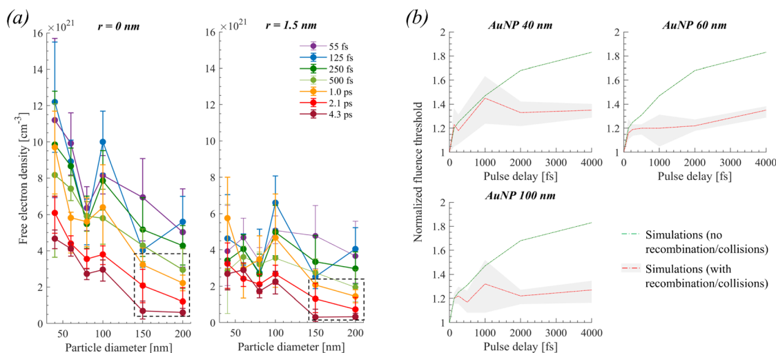
Fig. 4 (a) Maximum (in time) electronic densities calculated at the experimental fluence thresholds, at the poles of the particles ( r = 0 \text{ nm} ), and at a distance ( r = 1.5 \text{ nm} ) away from the pole. Dashed boxes indicate conditions where photothermal effects influence bubble formation (as demonstrated below in Fig. 5). (b) Calculation of required fluence threshold after double 55 fs pulse excitation as a function of pulse delay. The data of (a), for r = 0 \text{ nm} , was used as a reference to estimate by numerical simulations the theoretical normalized fluencies of the double pulse experiments shown in panel (b). Particularly, in (b), for the green solid curves, we considered that under double pulse excitation, the electronic density calculated for a single 55 fs pulse must be attained at the detected thresholds. For the red solid curve (error shown by grey area) we considered that approximately the electronic densities calculated for a longer pulse (e.g., 1.0 ps) must be attained at the detected threshold when the delay between double pulses increases (e.g., at 1.0 ps delay), which accounts for recombination/collision effects before the arrival of the second 55 fs pulse.
