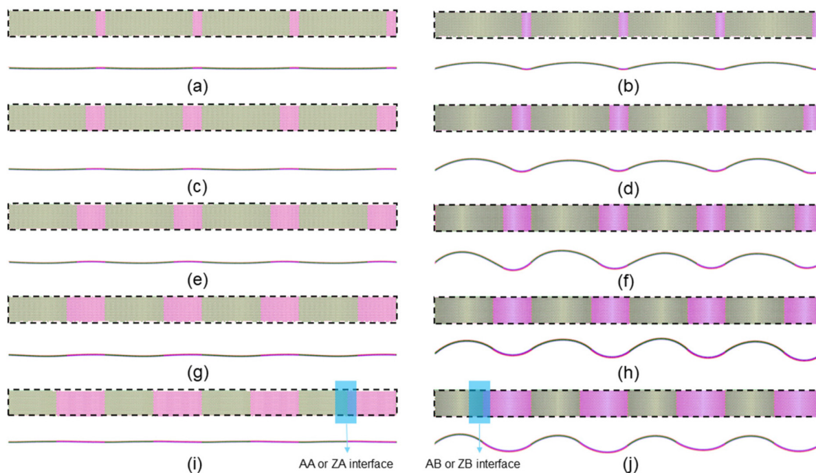
Fig. 2 The top and side views of optimized (a, c, e, g, and i) AA and (b, d, f, h, and j) AB Janus MoSSe/WSe heterostructures with L_m/L_n as (a and b) 1/9, (c and d) 2/8, (e and f) 3/7, (g and h) 4/6, (i and j) 5/5, respectively.
