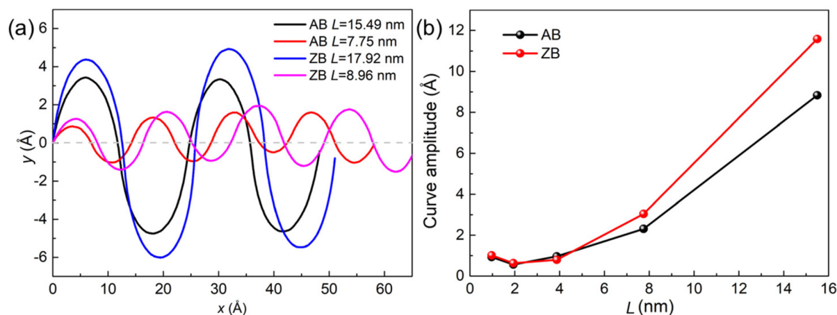
Fig. 3 (a) The fitted Fourier curve for the structural trajectory of the MoSSe/WSe heterostructure superlattice and (b) the amplitude value of the Fourier curve versus L .
