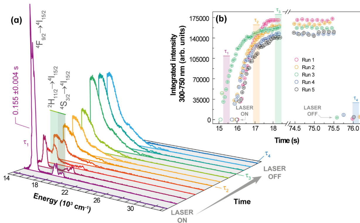
Fig. 6 Emission spectra of 1 acquired at 102 \text{ W cm}^{-2} under ambient conditions. (b) Transient integrated intensity over 300 at 750 nm (see text for the meaning of \tau_1 , \tau_2 , \tau_3 , and \tau_4 ).
