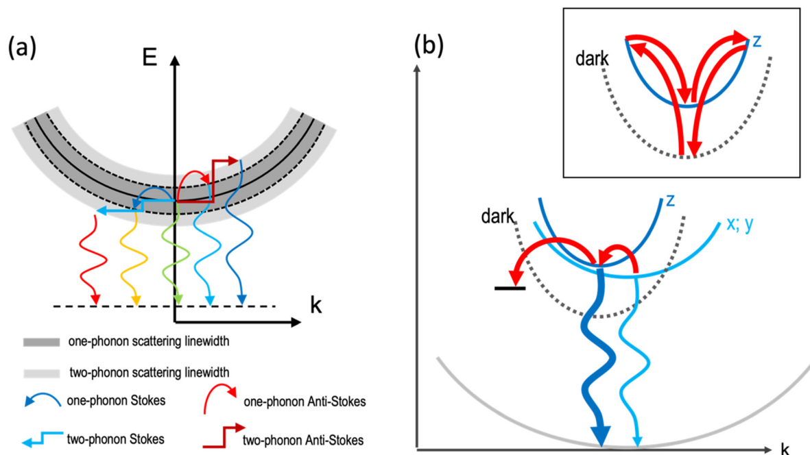
Fig. 2 (a) Illustration of the one-phonon and two-phonon scattering of excitons that leads to the emission linewidth broadening. One-phonon scattering is illustrated by the bend arrows, two-phonon scattering by the rectangular arrows, and emissive recombination is sketched by the waveform arrows. (b) Illustration of the phonon coupling between the bright emitting states and non-radiative defect states. The distortions induced by the organic cations lead to small offsets of the minima of the dispersions in k -space. The stronger quantum confinement in z -direction results in a stronger curvature of the dispersion. The dark exciton level is sketched by a dashed line and the radiative recombination by waveform blue arrows. The thicker line width of the dark blue arrow indicates the brighter emission of the HE band edge peak with respect to the low-energy ( x,y ) transitions. Phonon-assisted thermal transitions are sketched by the curved red arrows. The inset illustrates the two-phonon coupling between the dark state and the bright z -state. 16
