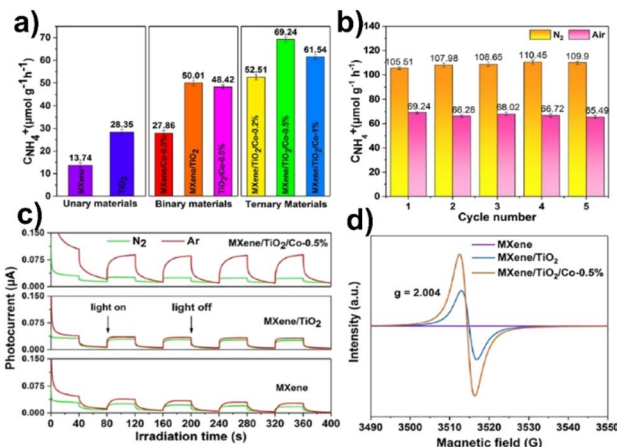
Fig. 12 (a) \text{NH}_4^+ production rate in ambient air; (b) the stability of N 2 photofixation activity of MXene/TiO 2 /Co-0.5% under N 2 and an air atmosphere; (c) photocurrent spectra of MXene, MXene/TiO 2 and MXene/TiO 2 /Co-0.5%; (d) EPR spectra. Reproduced with permission from ref. 163, Copyright 2015 American Chemical Society.
