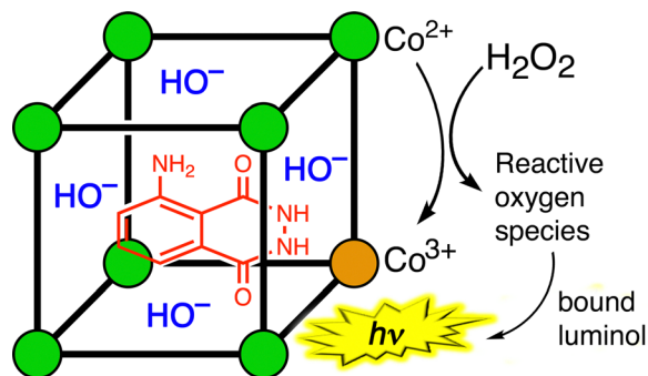
Fig. 12 Cartoon representation of the oxidation of luminol by \text{H}_2\text{O}_2 catalysed by the cage \text{H}^{12} which (i) binds the guest, (ii) uses its \text{Co(II)/Co(III)} redox couple to activate the \text{H}_2\text{O}_2 generating reactive oxygen species surrounding the cage surface, and (iii) tethers any hydroxide ions required for the reaction in place via the cage positive charge.
