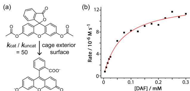
Fig. 3 (a) \text{H}^\text{W} -catalysed hydrolysis of diacetyl fluorescein; (b) dependence of the reaction rate on substrate concentration, fitted to a Michaelis-Menten reaction model to extract an association constant for the interaction between substrate and cage exterior surface (see main text).
