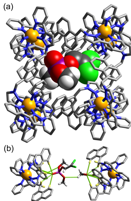
Fig. 2 Crystal structure of the \text{H} \cdot \text{dichlorvos} complex. (a) A view of the complete cage with the guest shown in space-filling mode; (b) a view of the guest (plus a MeOH molecule) emphasising the \text{CH} \cdots \text{O} interactions with the cage interior surface (green dotted lines).
