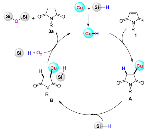
Scheme 3 Proposed mechanism for the \text{Cu}(\text{OTf})_2 @CAC-catalyzed selective reduction of maleimides.
