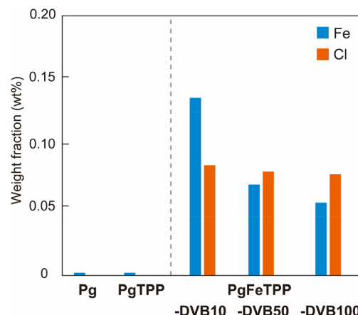
Fig. 5 Weight fraction of Fe and Cl in polymer powders measured by X-ray fluorescence analysis. Blue and orange bars indicate Fe and Cl, respectively.
