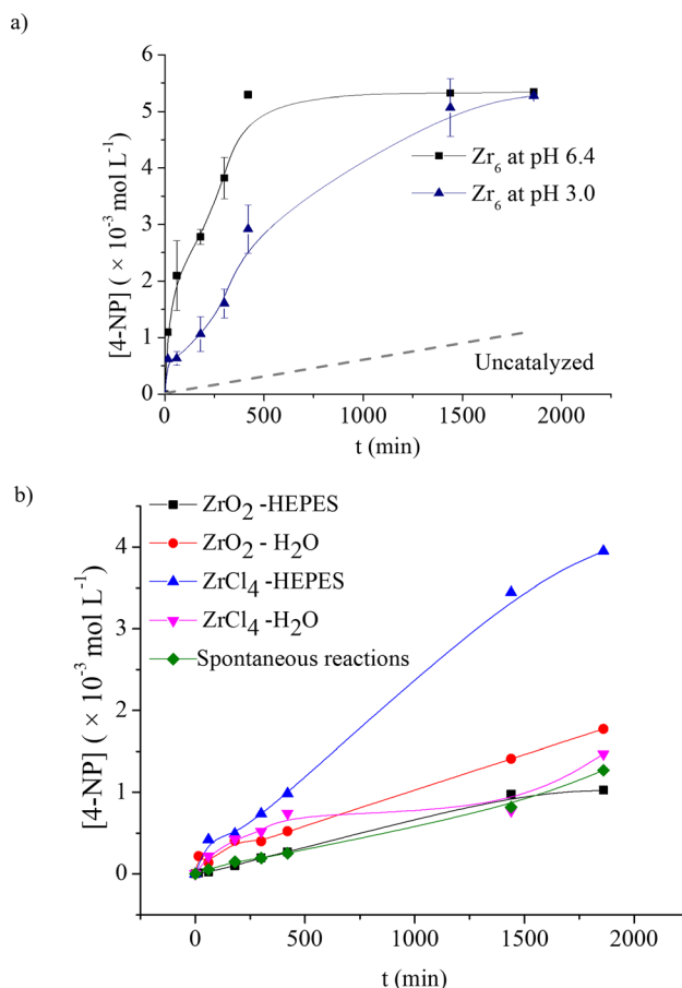
Fig. 3 (a) \text{Zr}_6 catalyzed hydrolysis of 1 at 60 °C and pH 3.0 (blue \blacktriangle ) and 6.4 ( \blacksquare black). Conditions: [\text{Zr}_6] = 1.5 \text{ mmol L}^{-1} ; [1] = 25 \text{ mmol L}^{-1} ; solvent (1 mL – water (pH 2.7–3.0) or HEPES 0.1 \text{ mol L}^{-1} (pH 6.4–6.7)); 60 °C. (b) Control experiments featuring hydrolysis of 1 at 60 °C catalyzed by Zr salts ( \text{ZrO}_2 and \text{ZrCl}_4 ) at pH 3.0 ( \text{ZrO}_2 – red circles \bullet ; \text{ZrCl}_4 – pink triangles \blacktriangledown ) and pH 6.4 ( \text{ZrO}_2 – black squares \blacksquare ; \text{ZrCl}_4 – blue triangles \blacktriangle ). Spontaneous hydrolysis at both pH 7.0 (HEPES 0.1 \text{ mol L}^{-1} ) and pH 3.0 is presented by green squares ( \blacklozenge ). Conditions: [\text{ZrCl}_4] = [\text{ZrO}_2] = 1.5 \text{ mmol L}^{-1} ; [1] = 25 \text{ mmol L}^{-1} ; solvent (1 mL – water (pH 2.7–3.0) or HEPES 0.1 \text{ mol L}^{-1} (pH 6.4–6.7)); 60 °C.
