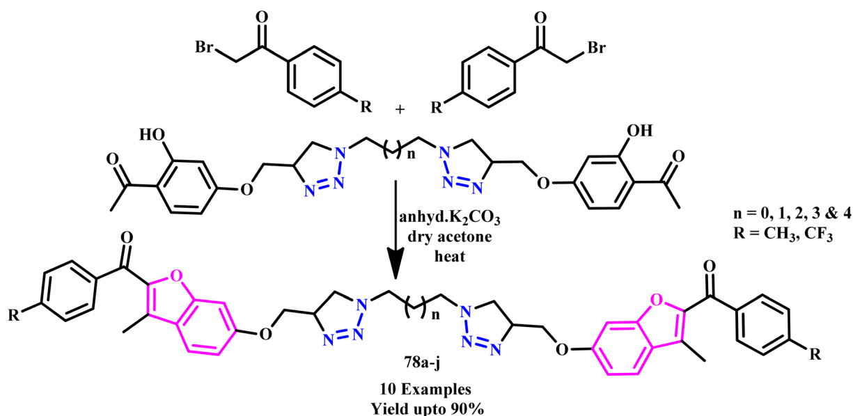
Scheme 67 Microwave-assisted synthesis of (6,6'-(1,1'-(propane-1,3-diyl)bis(1 H -1,2,3-triazole-4,1-diyl)bis(methylene)bis (oxy)(3-methyl-benzofuran-6,2-diyl)bis(4-substituted phenylmethanone))) (78a-j). 114
