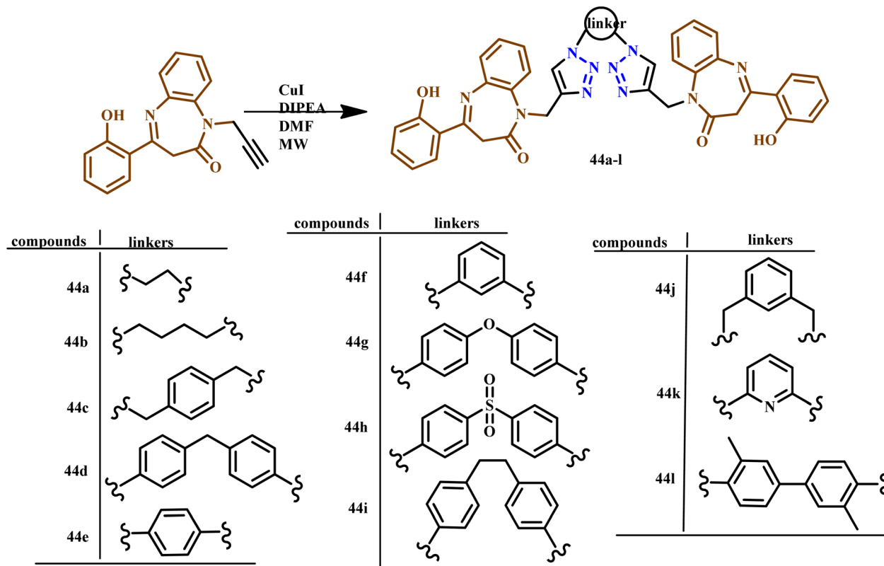
Scheme 33 Microwave-assisted synthesis of 1,1'-(1,1'-(hexane-1,6-diyl)bis(1H-1,2,3-triazole-4,1-diyl)) bis(methylene)) bis(1,5-benzodiazepin-2-one) and 1-((1-(6-azidoheptyl)-1H-1,2,3-triazol-4-yl)methyl)-(1,5-benzodiazepin-2-one) (44a-i). 73
