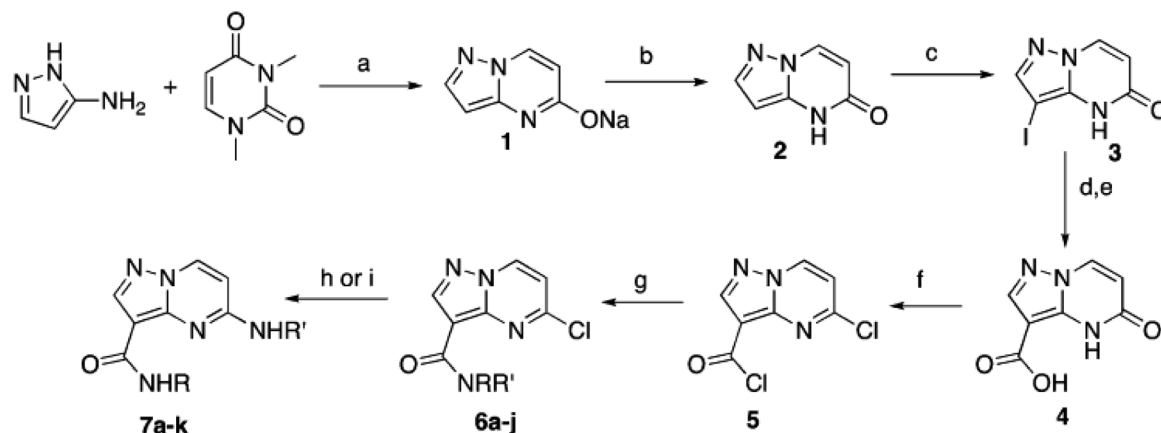
Scheme 31 General synthetic procedure for 5-amino-pyrazolo[1,5- a ]pyrimidine-3-carboxamides 257 Reaction conditions: (a) 21% EtONa, EtOH, 95%; (b) HOAc, H 2 O, 85%; (c) N -iodosuccinimide, DMF, 86%; (d) CO (1 atm), Pd(OAc) 2 , Et 3 N, MeOH; (e) 5% aq. LiOH, 68% (2 steps); (f) POCl 3 , DIPEA, 87%; (g) H 2 NR, DIPEA, DCM, 52–92%; (h) NH 3 , iPrOH, DIPEA, \mu W 120 °C, 15 min, 9–80%; (i) H 2 NCH 3 , H 2 O, \mu W 100 °C, 15 min, 62%. 257
