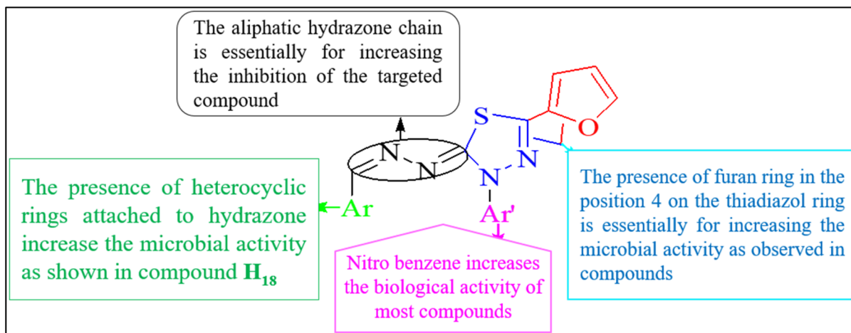
Fig. 5 Structure–activity relationship (SAR) of ( H_{16} – H_{18} ). 44
