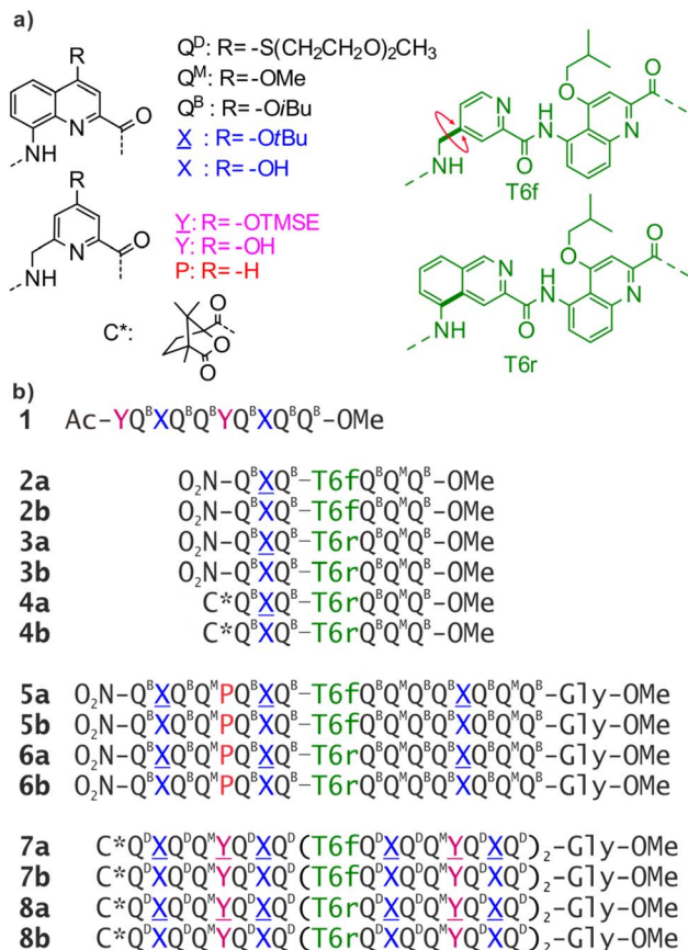
Fig. 1 (a) Structure of Q^D , Q^B , Q^M , X , Y , P , T6f, and T6r monomers as well as N-terminal chiral C^* group. X and Y are the hydroxy protected precursors of X and Y , respectively. TMSE = 2-trimethylsilyl-ethyl. (b) Oligoamide foldamer sequences. The Gly at the C terminus stands for glycine. In sequences ending with an 8-nitro group, this group replaces the terminal amine.
