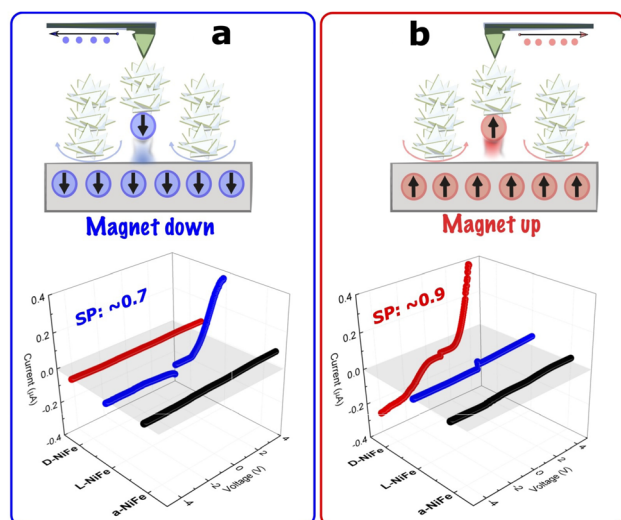
Fig. 5 mc-AFM-tip measurements with magnet down (a) and magnet up (b) for L-NiFe, D-NiFe, and a-NiFe catalysts. The current flow is indicated with arrows according to the magnetic field direction on the AFM tip.
