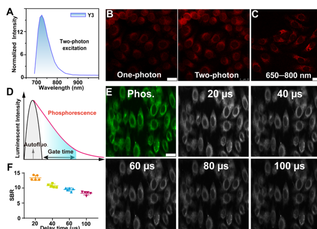
Fig. 6 Cellular two-photon and time-resolved imaging. (A) Two-photon excitation spectra of Y3 (0.1 mM) in water. (B) HeLa cells incubated with Y3 (50 \mu\text{M} ). One-photon imaging: \lambda_{ex} = 405 nm, \lambda_{em} = 580 – 700 nm. Two-photon imaging: \lambda_{ex} = 800 nm, \lambda_{em} = 580 – 700 nm, Scale bar: 25 \mu\text{m} . (C) NIR phosphorescence image of HeLa cells after incubation with Y3 (50 \mu\text{M} ), \lambda_{ex} = 405 nm, \lambda_{em} = 650 – 800 nm. (D) Schematic of organic RTP avoiding autofluorescence. (E) Time-gated luminescent images with various delay times of HeLa cells treated with Y3 for 4 h. Scale bar: 20 \mu\text{m} . (F) Phosphorescence intensity analysis of images in (E) with ImageJ software.
