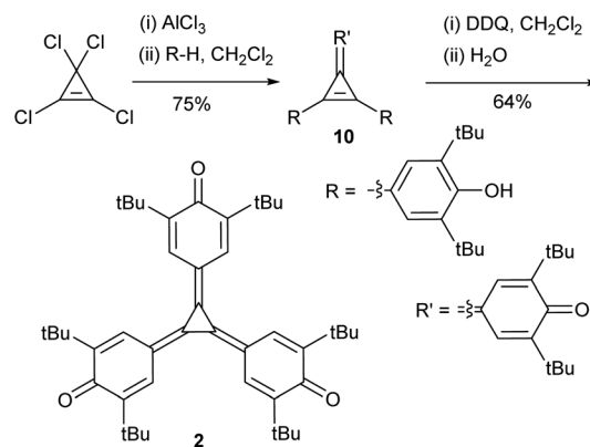
Scheme 1 Revised synthesis of triquino[3]radialene, which substitutes benzene and \text{PbO}_2 in the original for \text{CH}_2\text{Cl}_2 and DDQ, respectively.
