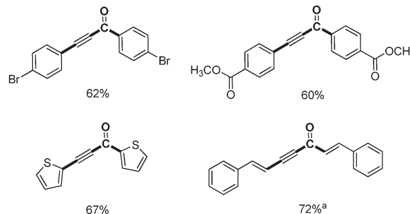
Scheme 32 One-pot synthesis of diaryl alkynones. a β-Bromostyrene was used.
