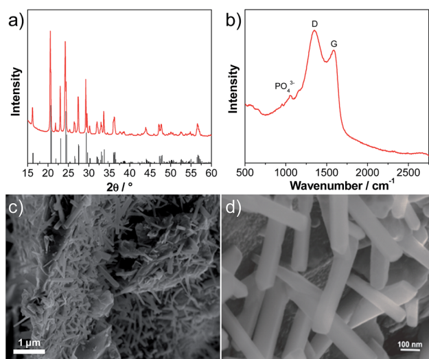
Fig. 1 (a) Powder XRD pattern (the reference for monoclinic \text{Li}_3\text{V}_2(\text{PO}_4)_3 (JCPDS card no. 96962) is shown in the bottom), (b) Raman spectrum and (c and d) SEM images of the nanostructured \text{Li}_3\text{V}_2(\text{PO}_4)_3 (LVP).
