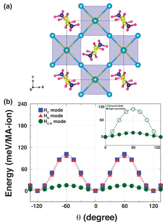
Fig. 3 (a) A high-symmetry structure characterised by the removal of octahedral tilting in o-MAPbI 3 . (b) The K–S energies plotted as a function of the torsion angle \theta for three rotational modes in the high-symmetry structure. Inset compares the energy barriers for the H C–N mode in the high-symmetry structure and the ground-state structure with octahedral tilting.
