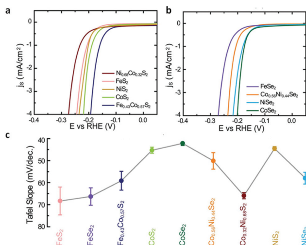
Fig. 10 (a) Polarization curves of transition-metal disulfides. (b) Polarization curves of transition-metal diselenides. (c) Summary of Tafel slopes of transition-metal dichalcogenide films (reproduced with permission from ref. 40. Copyright 2013 The Royal Society of Chemistry).
