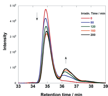
Fig. 6 Size exclusion chromatograms of the solutions before and after the photocatalytic reaction using \text{Ru}(\text{CH}_2\text{OCH}_2)\text{Re} (irradiation times: 0, 80, 120, 160, and 200 min). The eluent was \text{MeCN}-\text{MeOH} (1 : 1 v/v) containing 0.5 M \text{CH}_3\text{COONH}_4 ; two Shodex PROTEIN KW402.5 columns were used with a KW-LG guard column under the following conditions: flow rate, 0.2 \text{mL min}^{-1} ; column temperature, 40 ^\circ\text{C} ; detection wavelength, 390 nm. The reaction conditions were the same as those described in Fig. 5.
