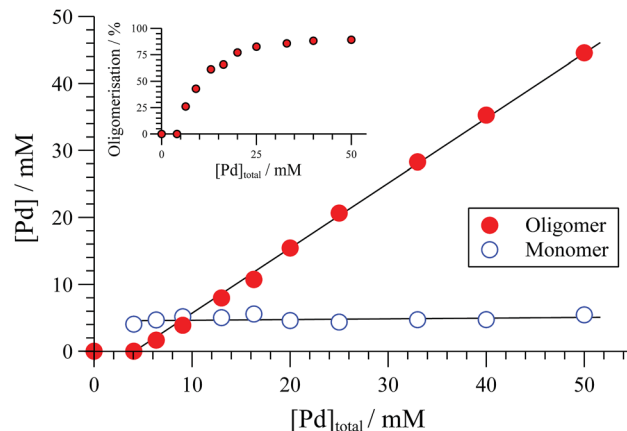
Fig. 1 Speciation of [( R,R )-1][BAR F ] (BAR F = B(C 6 F 5 ) 4 ) determined by 31 P{ 1 H} NMR (CD 2 Cl 2 , 25 °C). Solid lines through data are solely a guide to the eye. Inset shows proportion (%) of [Pd] tot that is in oligomeric form.
