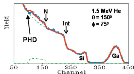
Fig. 6 Non-linearity of the RBS spectrometer. The sample is a 75 \times 10^{15} Ga cm ^{-2} implant at 75 keV into a 125 nm SiN _x :H thin film grown on Si. The detector is placed at a backscattering angle of 150^\circ and the sample normal is at 75^\circ to the beam direction. “Int” labels the SiN _x /Si interface as seen in the Si signal. The spectrum (red: calculated assuming linearity) fits the data (blue) perfectly except for the N interface signal (arrowed). “PHD” is the pulse-height defect (see text). Adapted with permission from Fig. 1 of Jeynes et al. , Anal. Chem. , 2012 73 (©2012, American Chemical Society); after Fig. 6 of Jeynes et al. , J. Phys. D: Appl. Phys. , 2003. 3 © IOP Publishing (reproduced with permission, all rights reserved); and redrawn from Nucl. Instrum. Methods Phys. Res., Sect. B , 148, Barradas et al. , RES and ERDA study of ion beam synthesised amorphous gallium nitride, 463–467, (©1999), 94 with permission from Elsevier.
