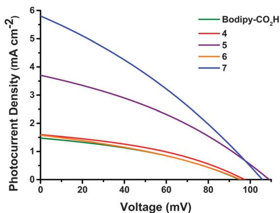
Fig. 3 Current-voltage characteristics of the dye-sensitized NiO solar cells with 0.1 M I _2 , 1.0 M LiI electrolyte and 4 (red), 5 (purple), 6 (orange), 7 (blue) and Bodipy-CO _2 H (green) under AM 1.5G (100 mW cm ^{-2} ) illumination.
